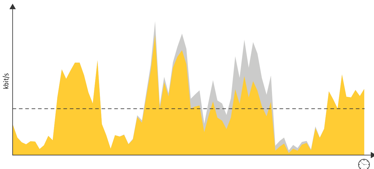
Figure 3.1 With ABR, a high image quality can be maintained during peak events thanks to savings from earlier, idle, periods. Averaged over a set period of time, the bitrate goal must be fulfilled.
