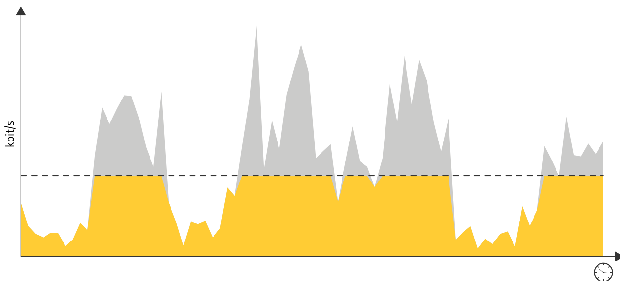
Figure 5.1 MBR, here illustrated with an aggressive bitrate limit. Storage requirements will be predictable, but information loss can be severe in complex scenes.
