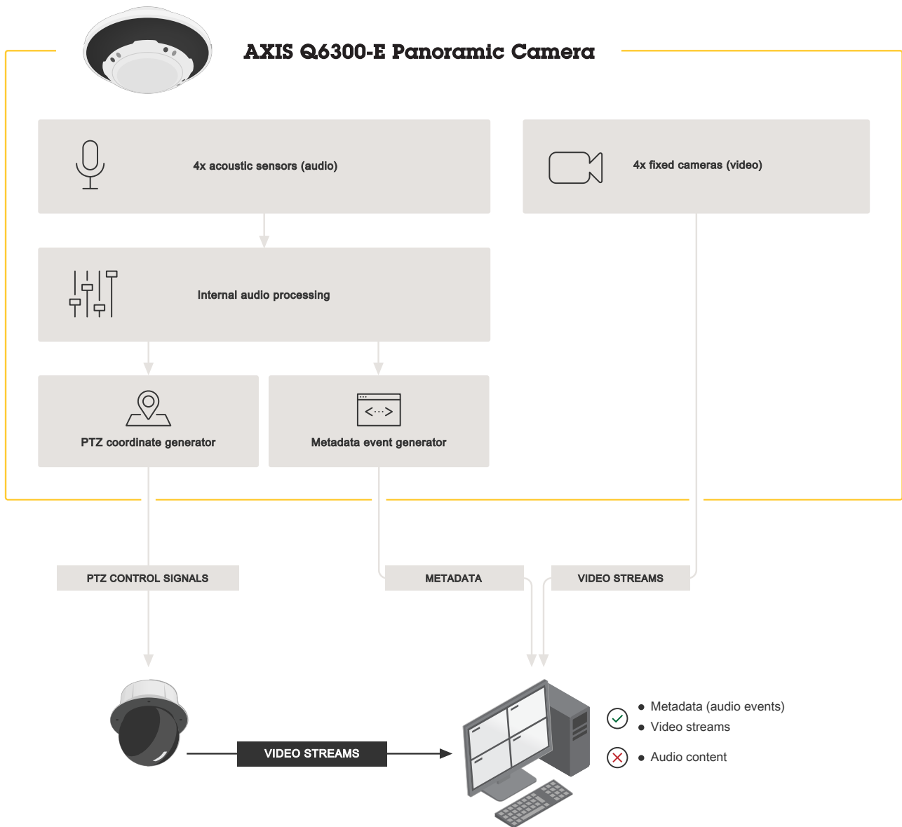
Figure 6.1 System architecture and data flow in directional audio detection. No audio content leaves the camera.
