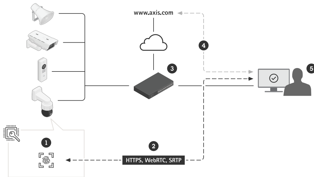
Figure 9. After a device has been securely onboarded, software applications (5) in other parts of the system can use the Axis device ID (1) and cryptographic operations to verify and authenticate the device in various TLS-based communication (2). The Axis device ID is verifiable by the publicly available Axis device ID root CA certificate (4).
