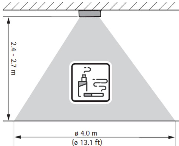
Coverage of a ceiling-mounted sensor for detection of smoking or vaping.
