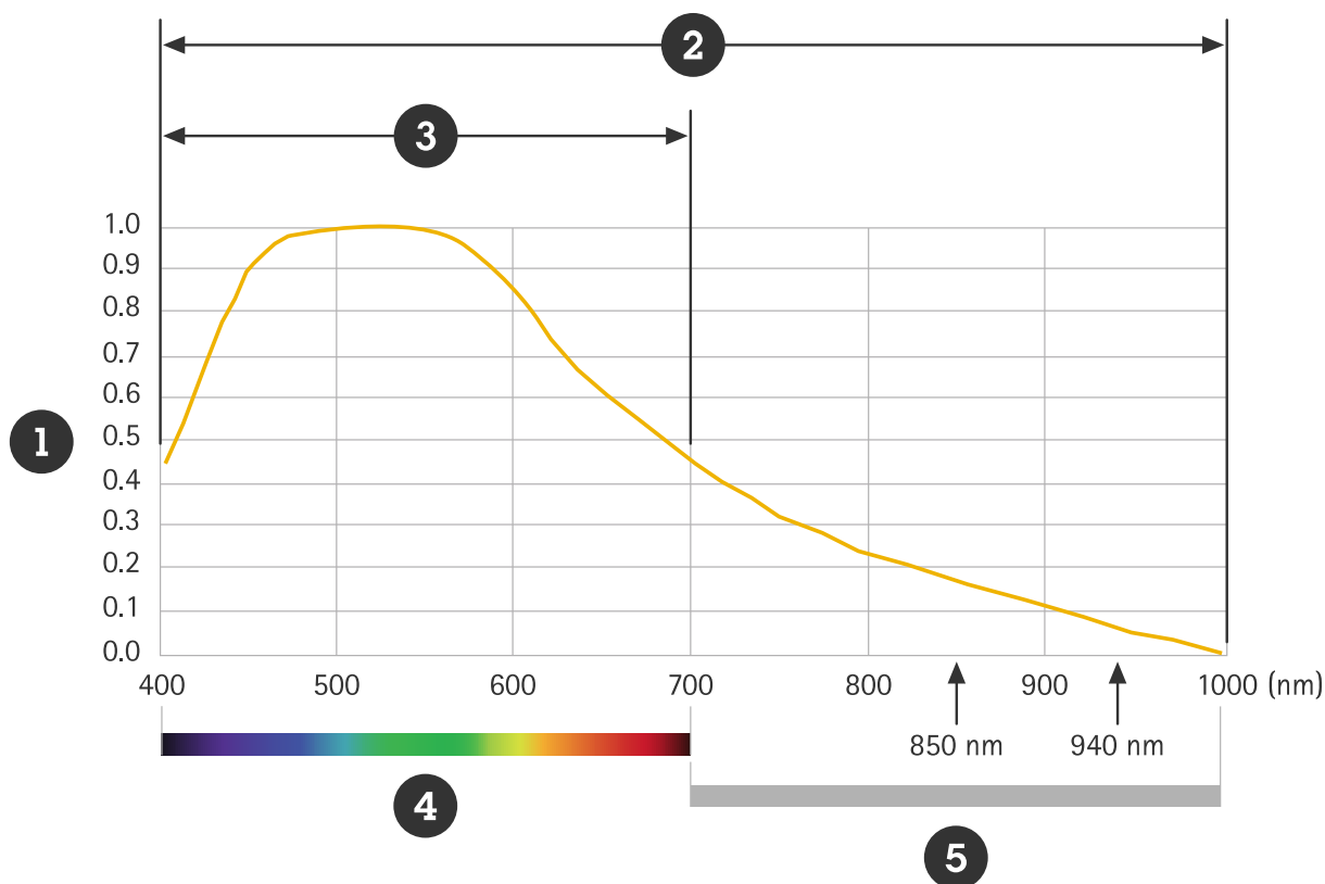
Image sensor response to visible and NIR light.
