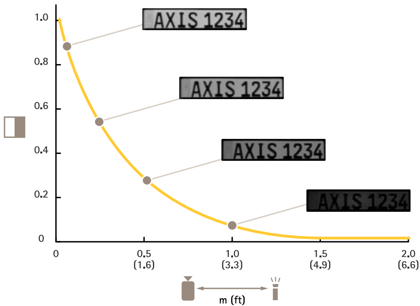
The relative contrast of a license plate 10 m (33 ft) away, as a function of the distance (perpendicularly to the road) between the camera and the external IR source.
