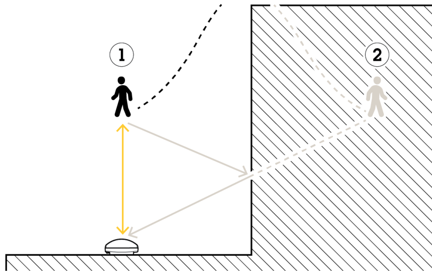
Figure 4.2 With walls or similar objects in the radar's range, false detections (2) caused by reflection can be difficult to separate from real detections (1). In this example, you could minimize the issue by adding an exclude zone around the wall.
