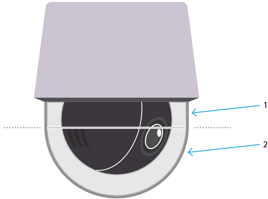
Figure 2.2 A conventional camera dome consists of a cylindrical part (1) above a half-spherical part (2).
