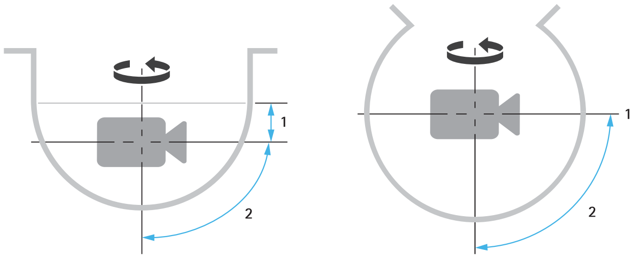
Figure 2.3 Placement of camera block in a conventional dome (left), and in an optimal dome (right). "1" marks the L-value (for an optimal dome, L=0 ) and "2" marks the 90^\circ tilt angle.
