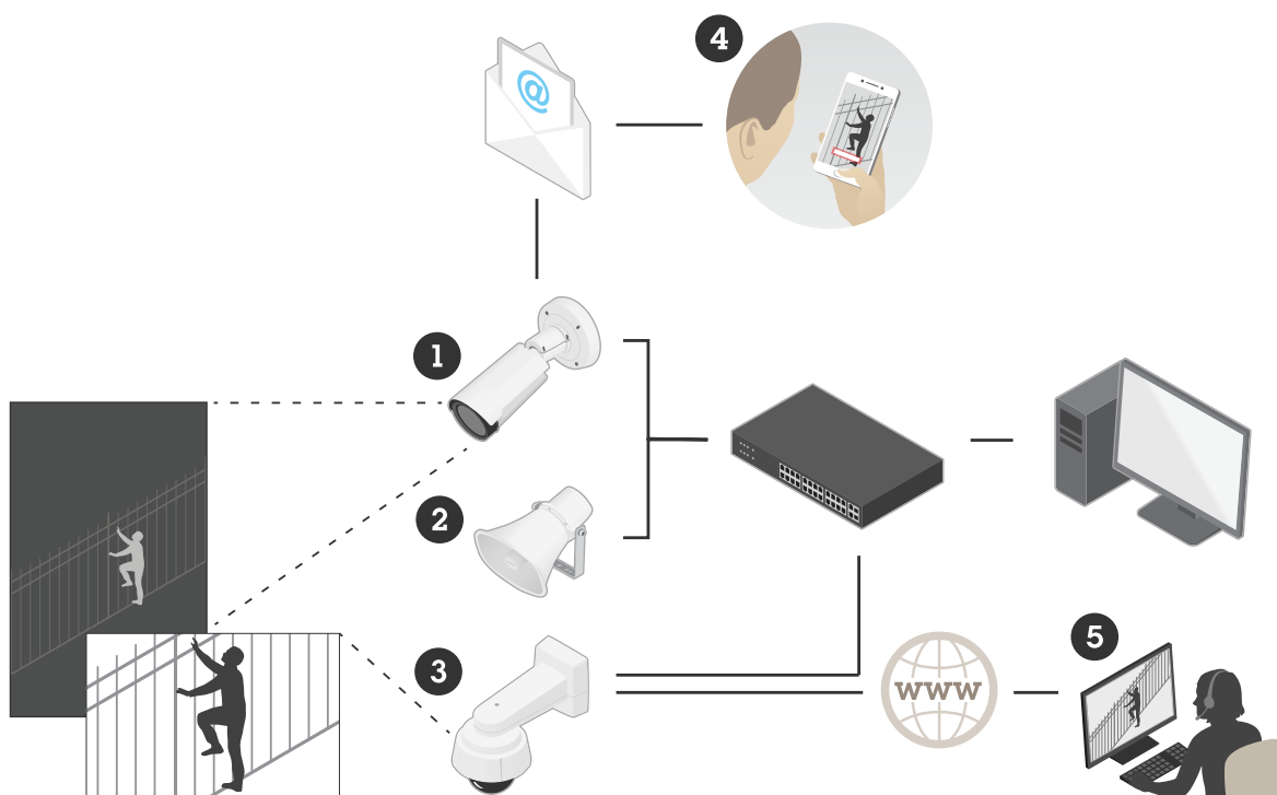
The role of a thermal camera in a perimeter protection system:
